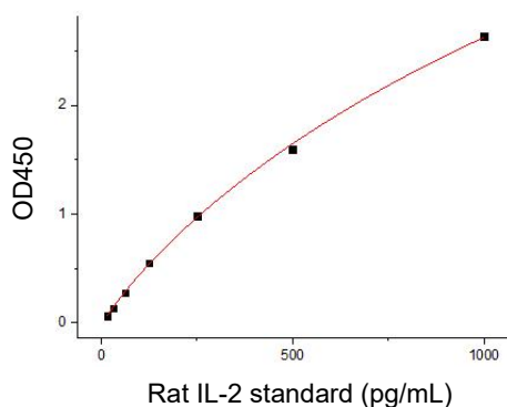
Figure1. Standard curve of Rat IL-2 in 96-well plate assay, data provided for demonstration purposes only. A new standard curve must be generated for each assay.
