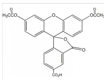
Fig. 5-CFDA structure formula
