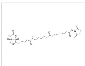
Fig. Biotin-XX, SE structure formula
