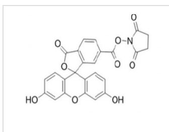
Fig. 6-FAM, succinimidyl ester structure formula
