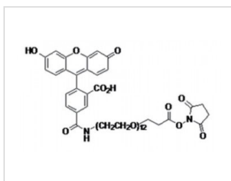
Fig. 5-FAM-PEO12, succinimidyl ester structure formula
