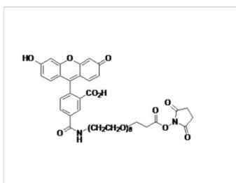
Fig. 5-FAM-PEO8, succinimidyl ester structure formula
