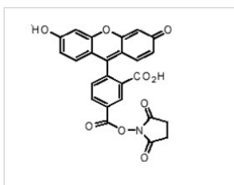
Fig. 5-FAM, succinimidyl ester structure formula
