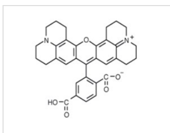
Fig. 6-ROX structure formula
