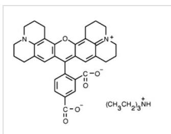
Fig. 5-ROX structure formula
