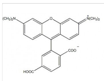
Fig. 6-TAMRA structure formula
