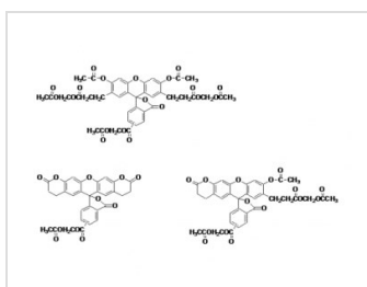
Fig. BCECF, AM ester structure formula
